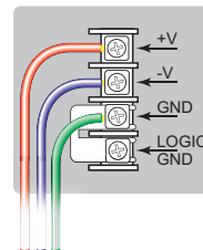
12-24 VDC 12-24VDC
