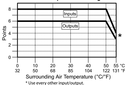
C0-00DR-D Temperature Derating Chart
