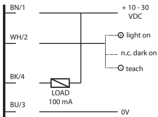
Diagram 3 4-Wire NPN Output DMP
