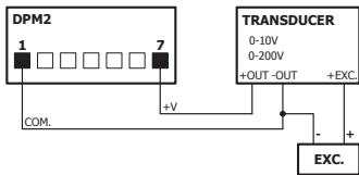
3 WIRE CONNECTION WITH EXTERNAL EXCITATION
